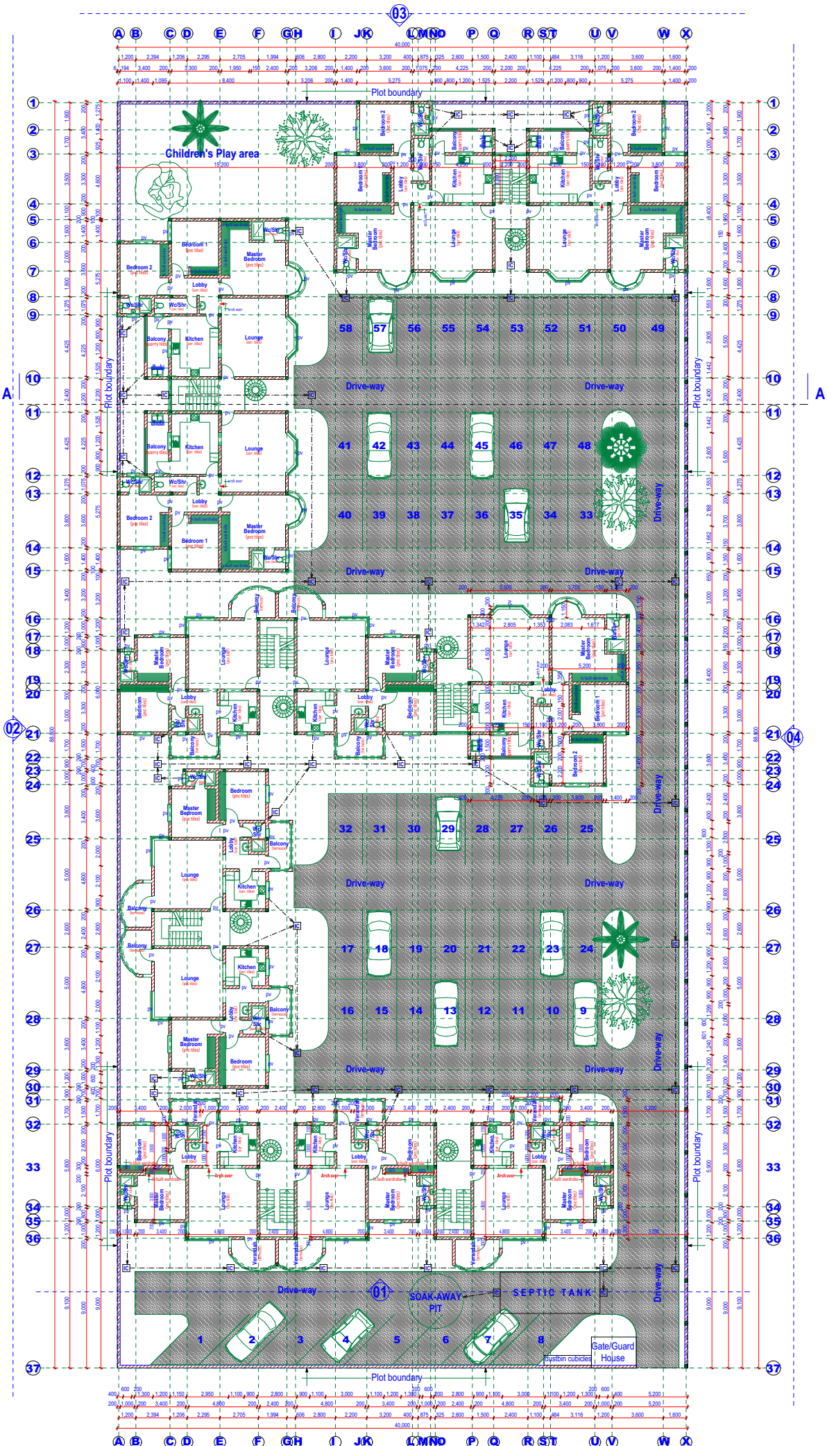
GROUND FLOOR LAYOUT PLAN
